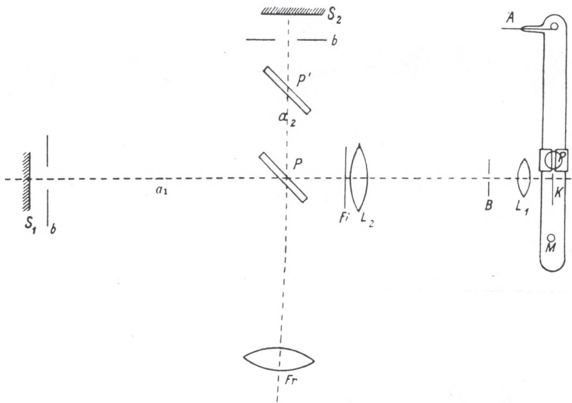
Figure 3. Rupp's original experiment for his Habilitation . Light enters the interferometer from the right, where it is emitted by canal ray light source at K . Source: Rupp 1926a.
