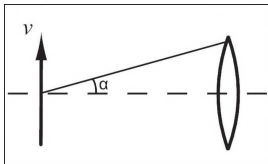
Figure 6. Doppler effect, with the canal ray beam moving up.
