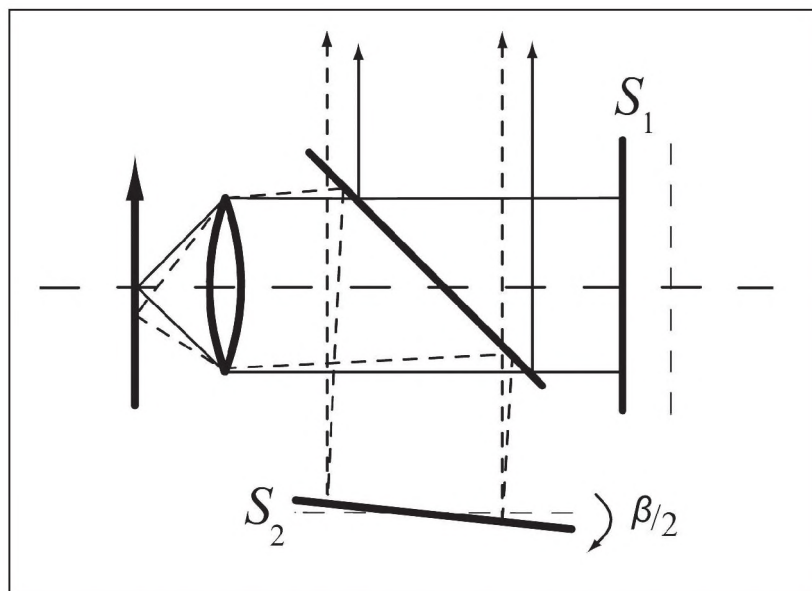
Figure 7. Due to the rotation of mirror S_2 , the interference pattern should be restored.
