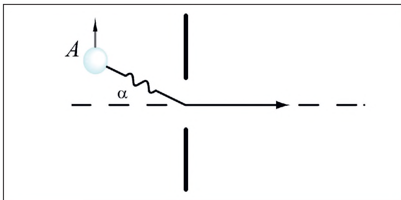
Figure 1. Atom A radiating behind a slit, with the emitted light undergoing diffraction.
